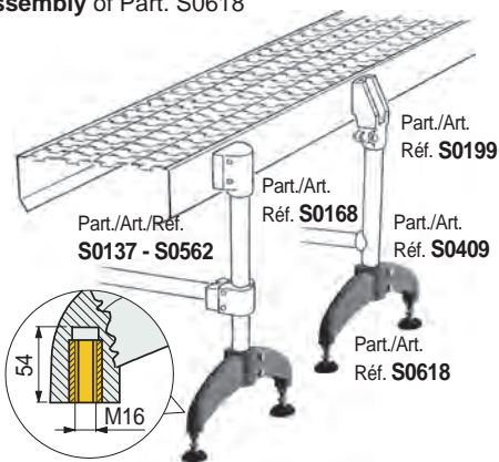
Detail of the insert for the levels.
